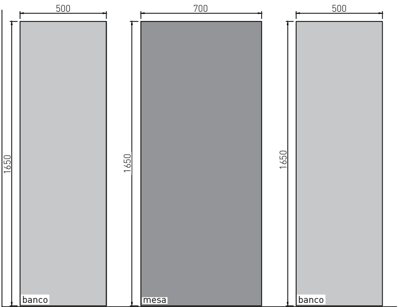
planta plan view
