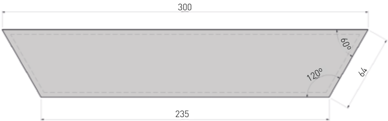
alzado frontal view
