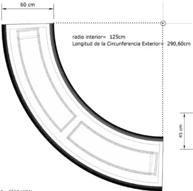
planta plan view
